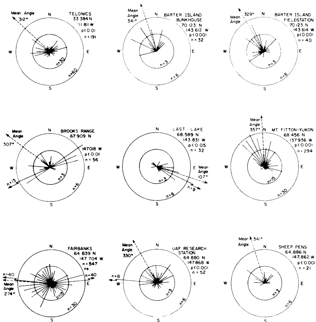
Fig. 31. Distribution of azimuths between the true location of a transmitter and the location calculated by Argos for nine sites. The mean angle and significance level (Hotelling's T^2 test for directional bias) is shown for each site.
