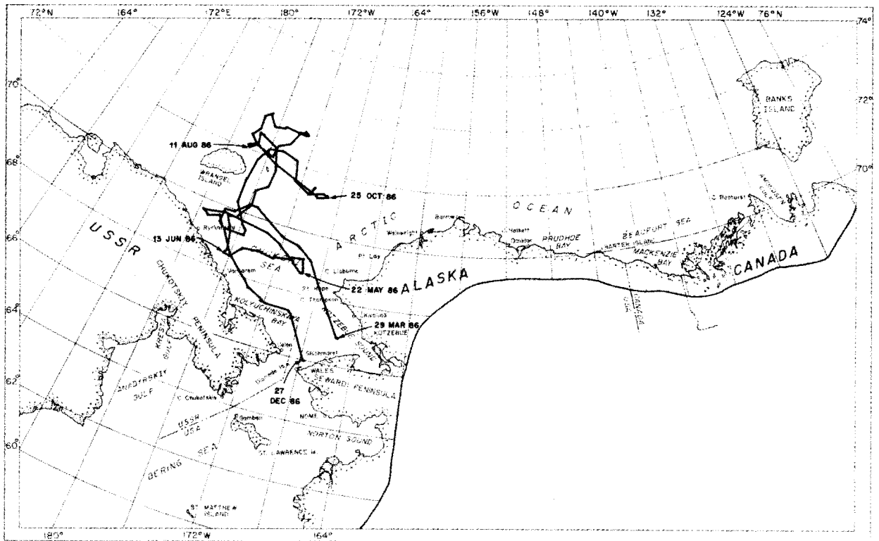
Fig. 40. Movements of a radio-collared female polar bear in the Chukchi Sea between March 1986 and December 1986.
