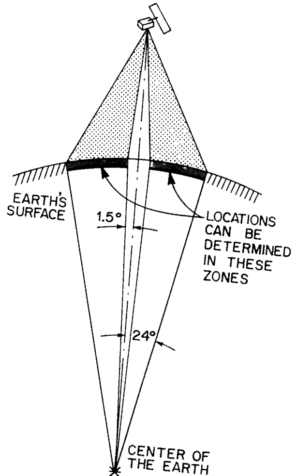
Fig. 20. Locations can be calculated for transmitters within a zone of approximately 170-2,700 km on either side of the satellite ground track. Locational errors are usually unacceptably high if the transmitter is outside these zones (adapted from Argos 1984).
