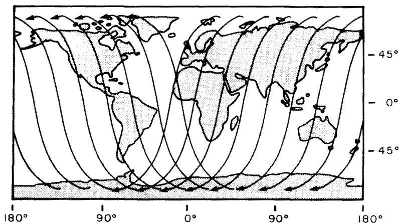
Fig. 7. Mercator projection showing the ground track of a Tiros-N satellite. The ground track at the equator is displaced 25° to the west with each revolution as a result of the earth's rotation during the 102-min period of the satellite.
