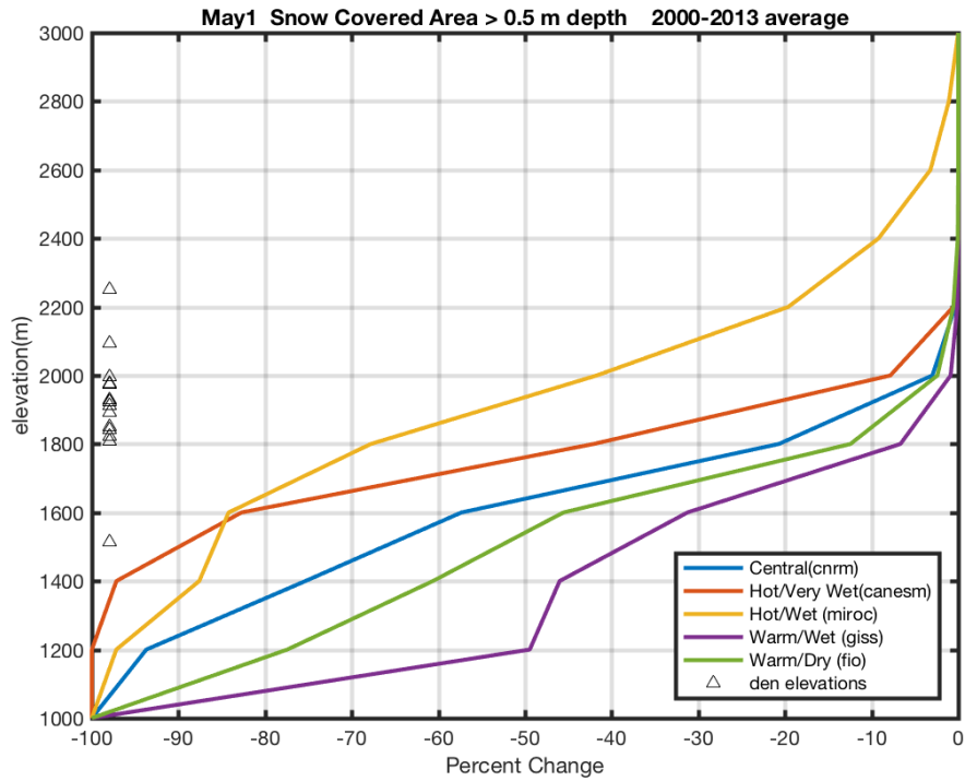
Figure 8. Average Snow Covered Area (depth ≥ 0.5 m (20 in)) percent change at elevation bands for GLAC for five future scenarios on May 1.
