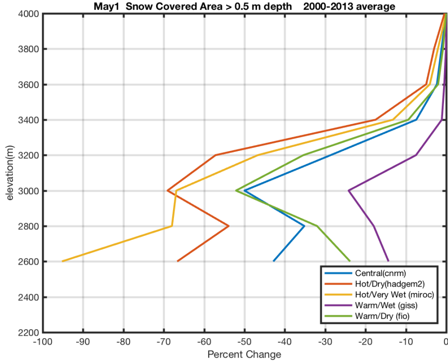
Figure 9. Average Snow Covered Area (depth ≥ 0.5 m (20 in)) percent change at elevation bands for ROMO for five future scenarios on May 1.
