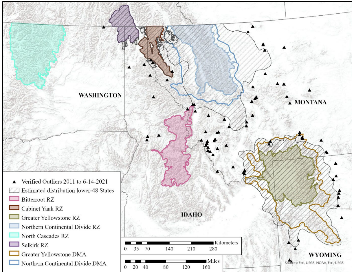
Figure 29. Estimated distribution of grizzly bears in the NCDE (2011–2020 data), GYE (2006–2020 data), CYE (2005–2019 data), and SE (2005–2019 data), and verified grizzly bear outlier observations between the ecosystems based on data from 2011 to June 14, 2021.
