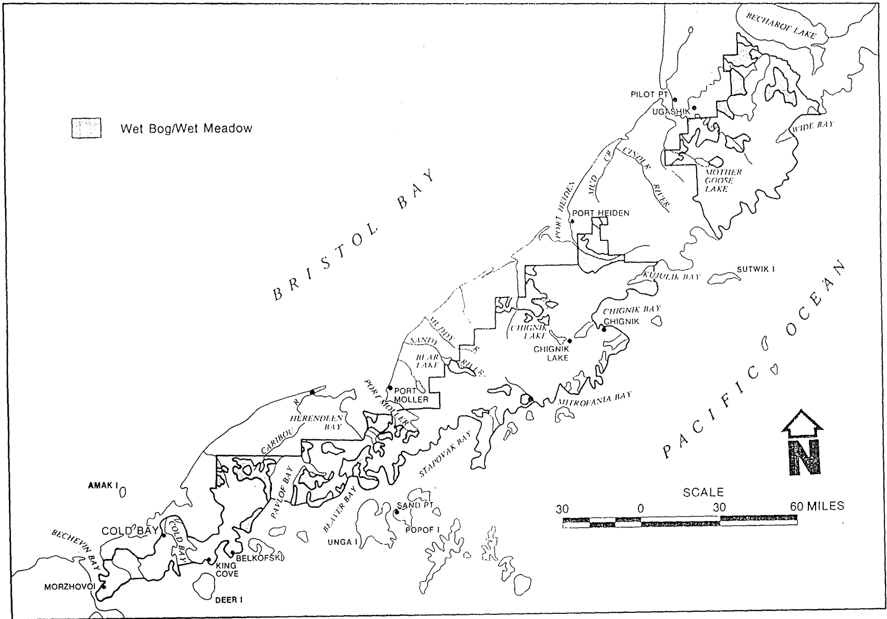
Figure 7. Cover types-wet bog/wet meadow.
