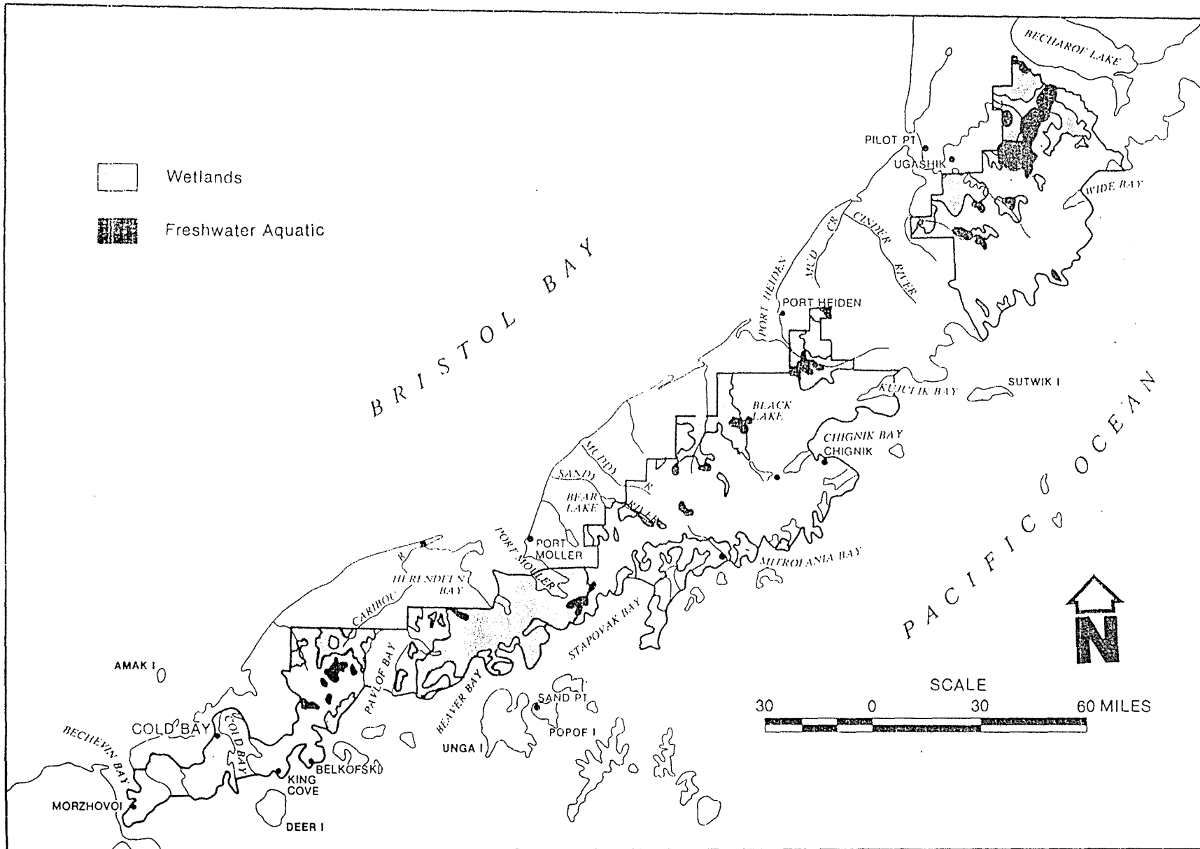
Figure 8. Ecosystems-wetlands and freshwater aquatic.
