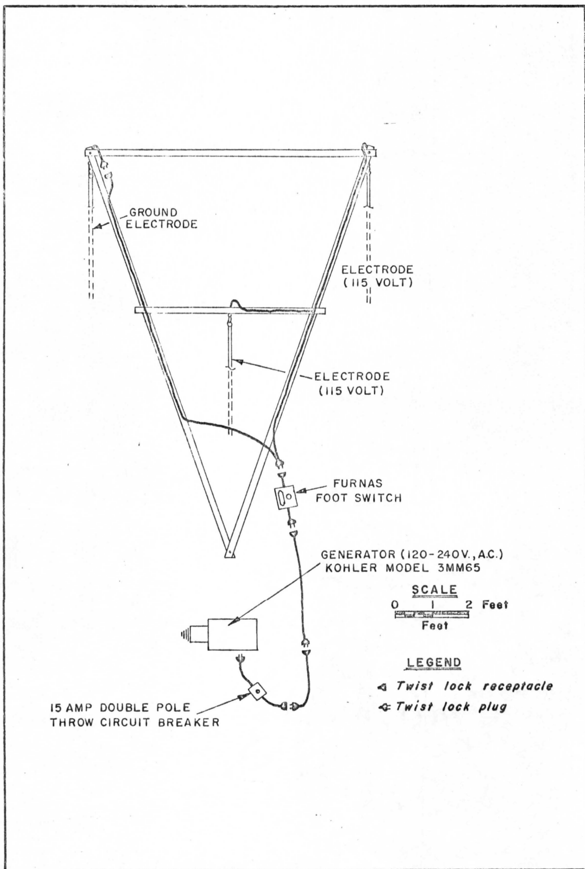
FIGURE 1 - A SCHEMATIC DIAGRAM OF A.C. SHOCKING UNIT USED
