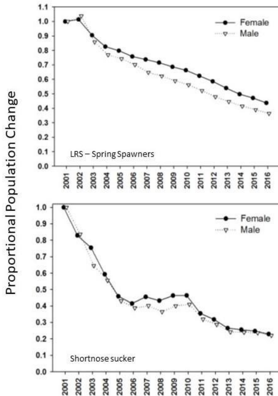
Figure 6-3. Adult spawning populations of suckers in UKL have consistently declined since at least 2001, as estimated by two approaches using mark-recapture models in Program MARK (from Hewitt et al. 2018 pp. 14 & 20). The number of spawning female LRS in UKL has declined by nearly 60 and SNS by 80 percent between 2002 and 2016.
