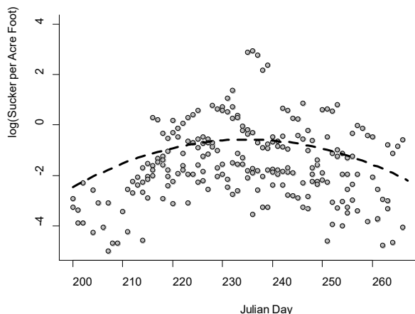
Figure A2. Fitted linear model (dashed line) and raw data for sucker density in catches at the Fish Evaluation Station across the season.
